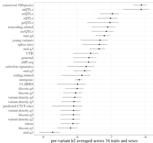
Fig. 3. The proportion of genetic variances explained by sets of variants selected from functional and evolutionary categories. The ranking of variant sets based on the \log_{10} scale of per-variant \bar{h}^2_{set} , averaged across bulls (left error bar) and cows (right error bar).
